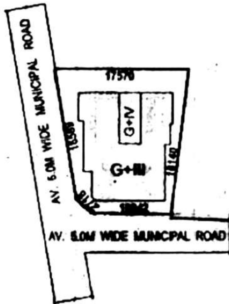
SITE PLAN
